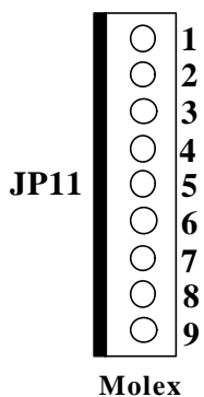
Figure 4-9 Reader 1 Connector
