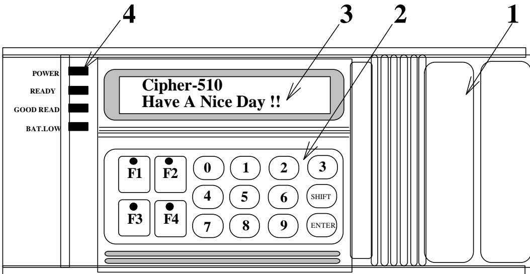
Figure 4-1 Main Panel
