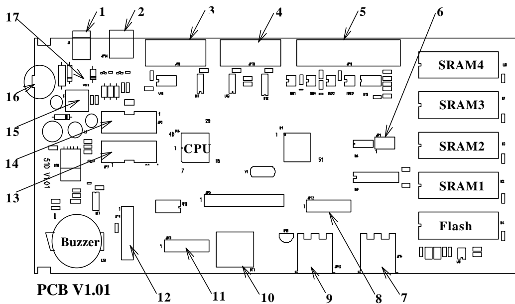
Figure 4-5 Left Panel
