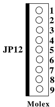
Figure 4-8 Reader 1 Connector
